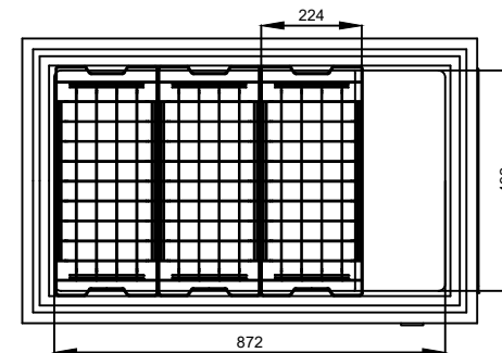
Top opened
