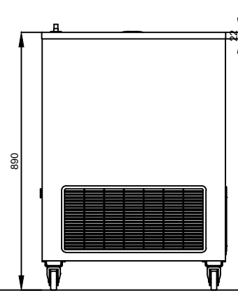
Right side
