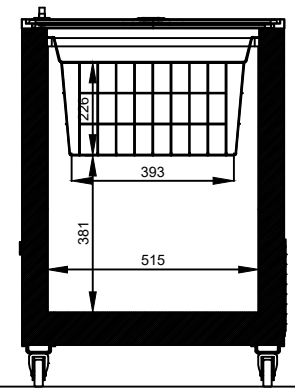
Section side
