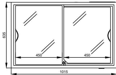
Top closed
