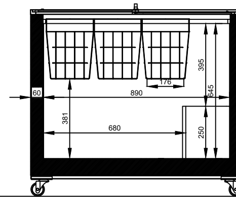
Section front
