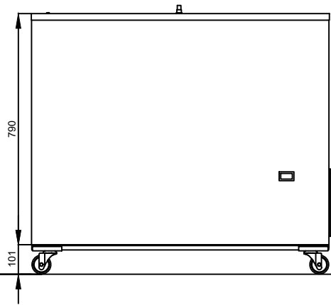
Top closed
